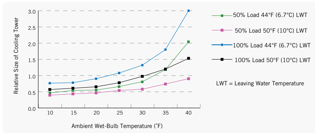
Figure 1. The Required Size of a Cooling Tower or Closed Circuit Cooling Tower Depends on the Load, Ambient Wet-Bulb Temperature, and Leaving Water Temperature
