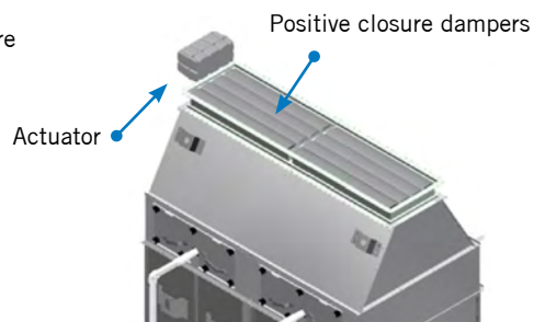
Figure 37b. Tapered discharge hood with positive closure dampers
