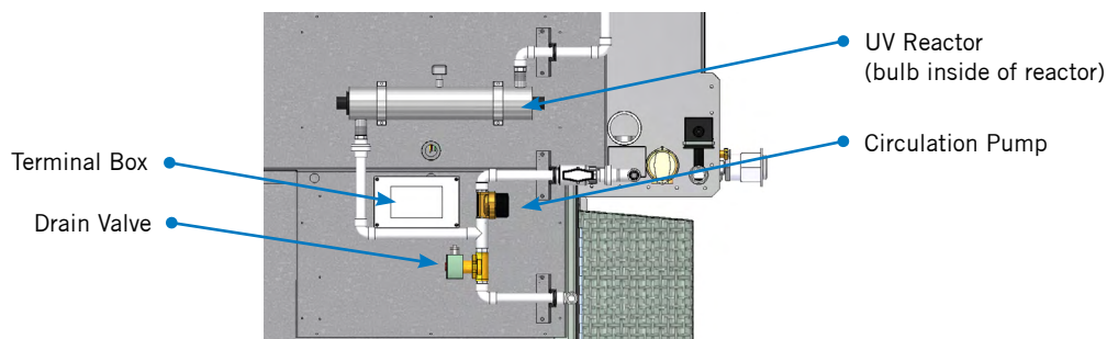
Figure 42. UV System components view
