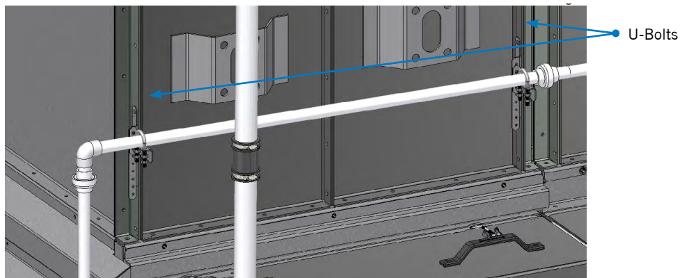
Figure 48. Crossover piping assembly
