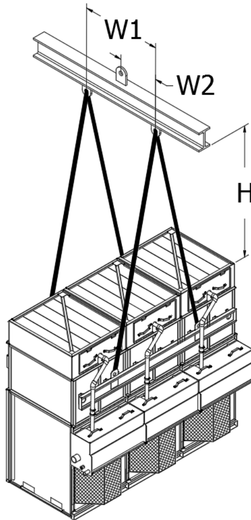
Figure 2. Lifting of Factory-Assembled Multi-Module Unit (Three Module Unit Shown)
