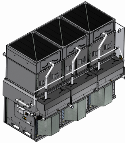
Figure 47. UV System crossover piping for multi-module units
