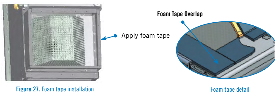
Figure 27. Foam tape installation
