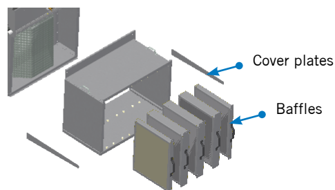
Figure 30. Baffle installation
