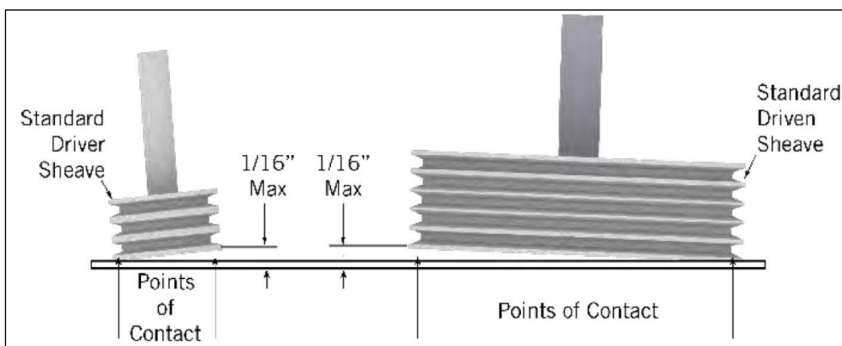
Figure 8. Drive Alignment
