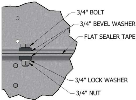
Figure 12. Detail A, Section Assembly
