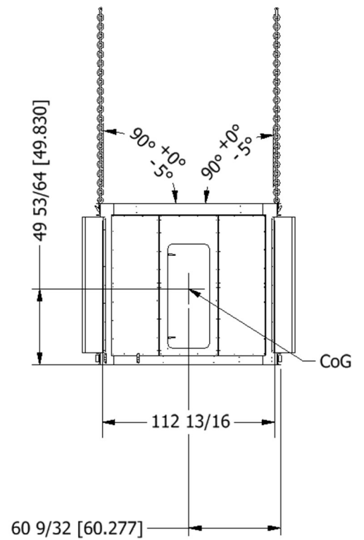
Figure 6. Lower Section Rigging Dimensions. Measurements are in inches.
