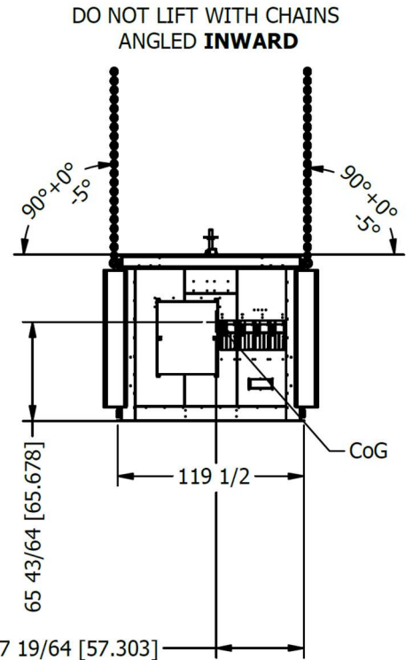
Figure 9. Upper Section Rigging Dimensions (units are inches)
