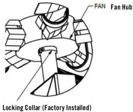
Figure 44: Bushing Keyway
