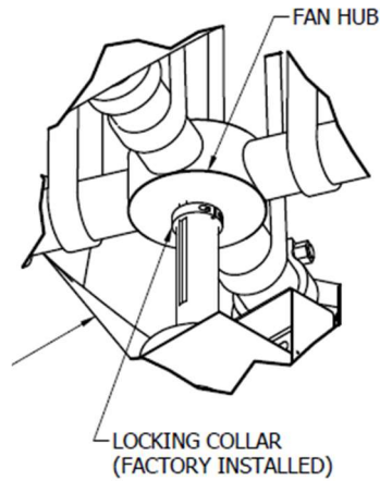
Figure 43: Hub detail
