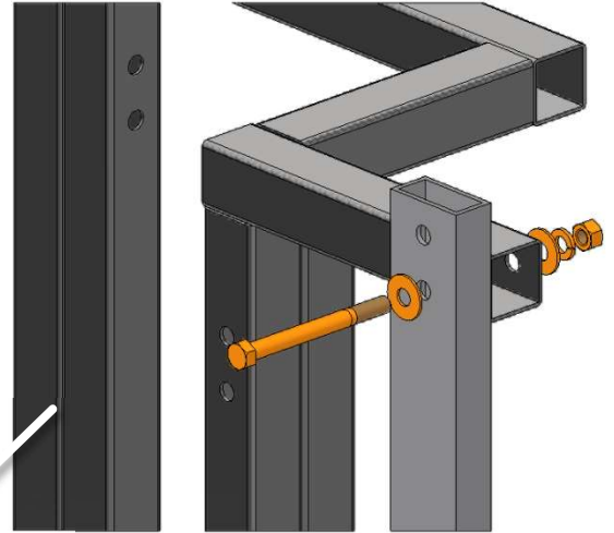
Figure 268. External Platform Ladder Flare to Railing
