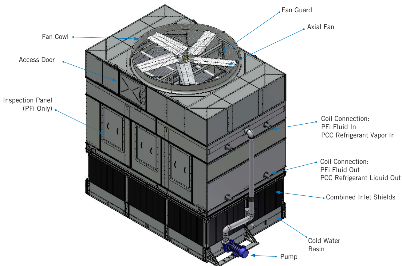
Figure 1. PFI Closed Circuit Cooling Tower and PCC Evaporative Condenser
