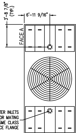
PLAN VIEW
