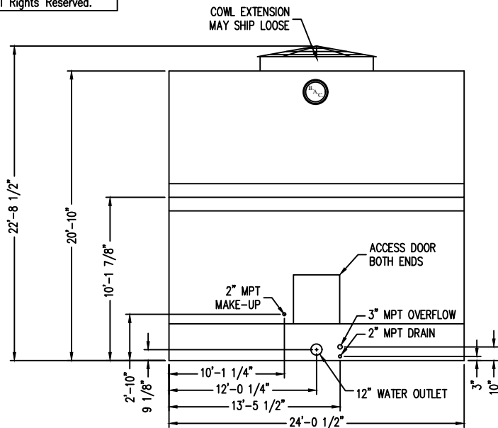
END ELEVATION (FACE A)
