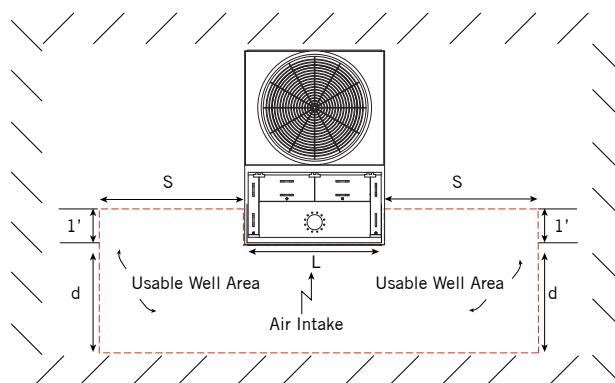
Figure 6. Plan View of Single Air Intake Unit in a Well Enclosure
