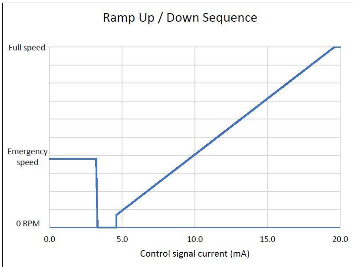
Figure 19. Ramp-up Sequence
