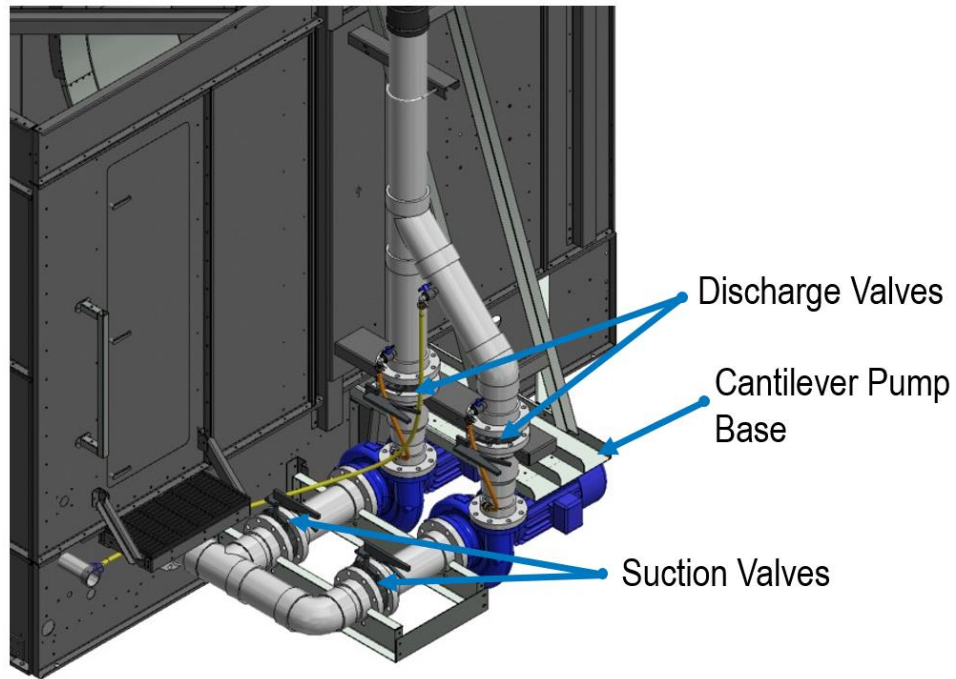
Figure 14. Discharge and Suction Valves
