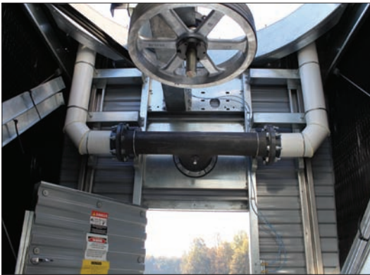
EASY CONNECT® Piping Arrangement
