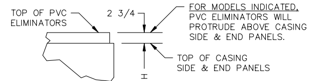
DETAIL "A"
