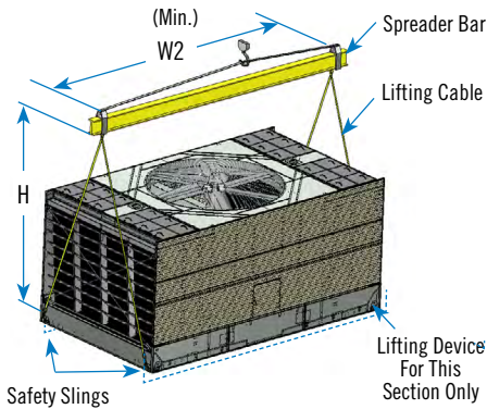
Figure 1b. Alternate Lifting Instruction: Air Intake Side (One Section Unit Shown)
