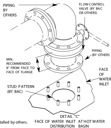
Figure 19. Piping Drawing Details
