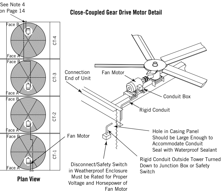
Figure 22. Motor Location For Close-Coupled Gear Drive
