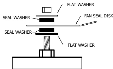
Figure 42. Replace Seal Disk
