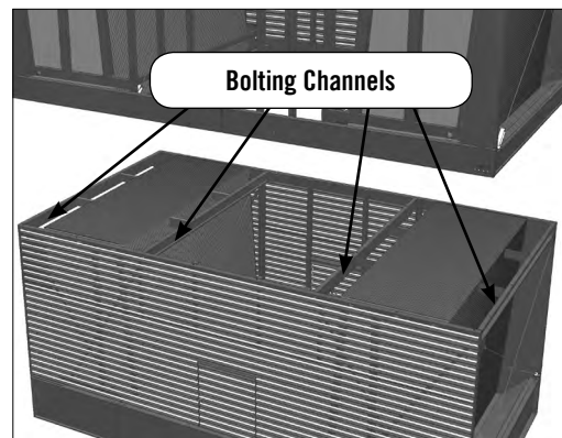
Figure 8. Bolting Channels
