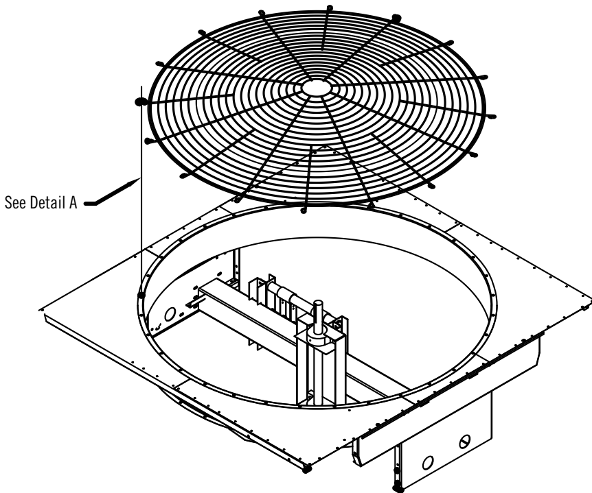
Figure 14. One-Piece Fan Guard Assembly
