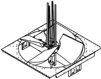
Figure 39. Fan Positioning
