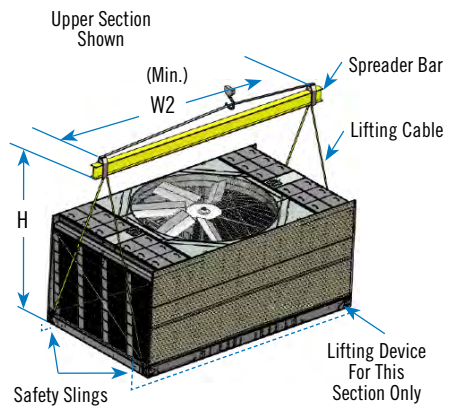
Figure 3b. Alternate Lifting Instruction: Air Intake Side (Two Section Unit, Upper Section Shown)
